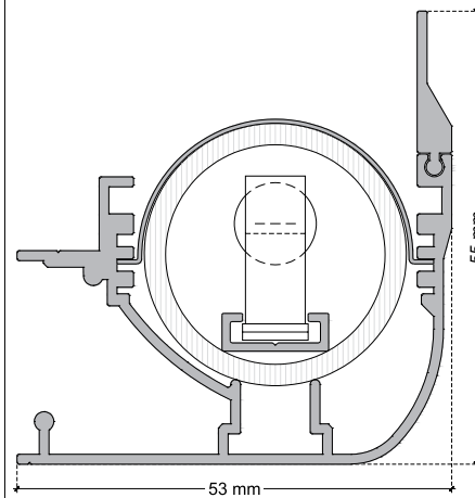
LU4TX66 + Tube Silicone / Xenon 3W/5W max.
